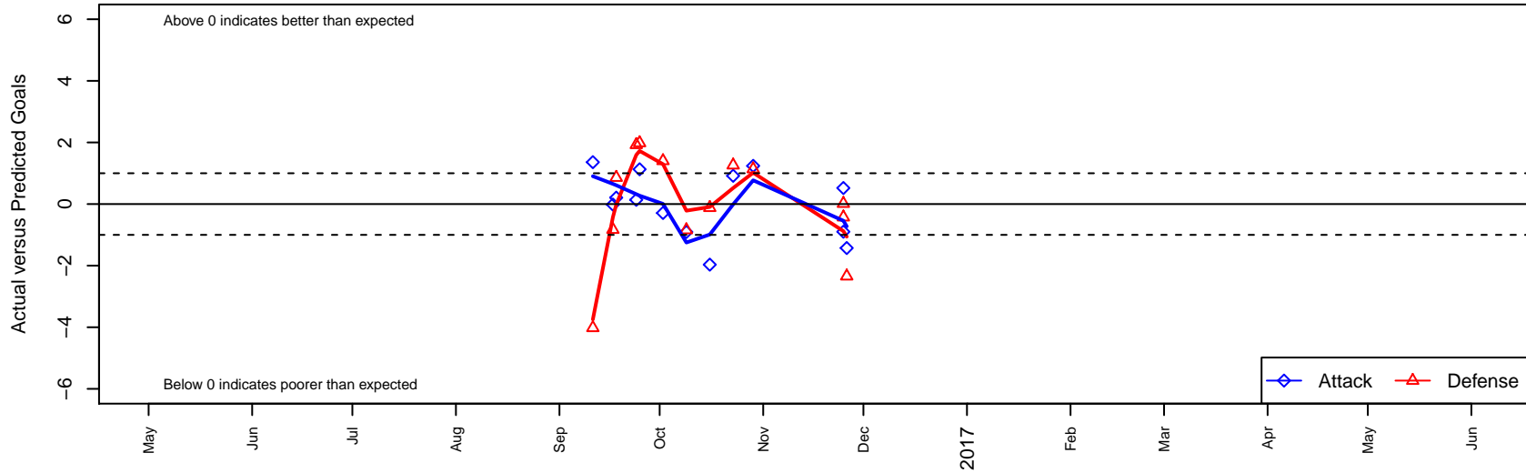
Pateadores Riverside B00 Dots are actual minus expected GF (blue circles) and GA (red triangles). Blue line is smoothed change in attack strength. Red is smoothed change in defense strength.
